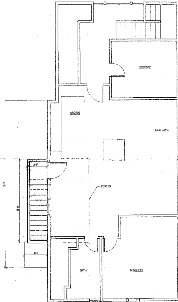
2 SECOND FLOOR PLAN 14-11-07
